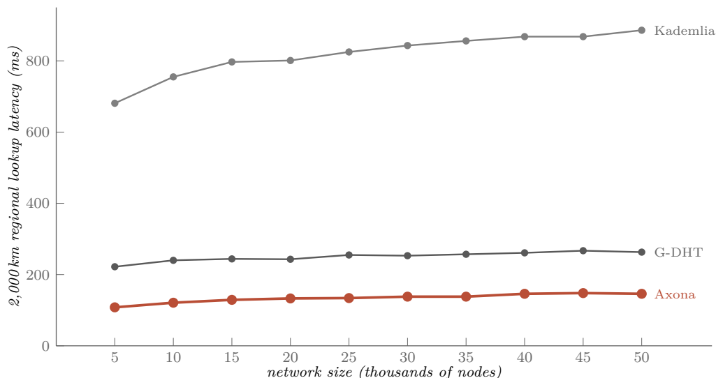
Figure 5: 2,000-kilometer regional lookup latency at every 5,000 from 5,000 to 50,000 nodes. Kademlia climbs from 681 to 886 ms—essentially the same as its global curve, because K-DHT has no way to know the lookup is regional and routes through full-planet hops anyway. G-DHT settles into a 222–267 ms band purely from the geographic prefix: \sim 3\text{--}3.4\times lower than Kademlia, with the curve nearly flat from 10,000 nodes onward. Axona drops further to 108–148 ms by layering learned per-hop locality on top of the structural prefix—roughly 1.8\text{--}2\times better than G-DHT and 6\text{--}6.3\times better than Kademlia. All success rates 100%.
