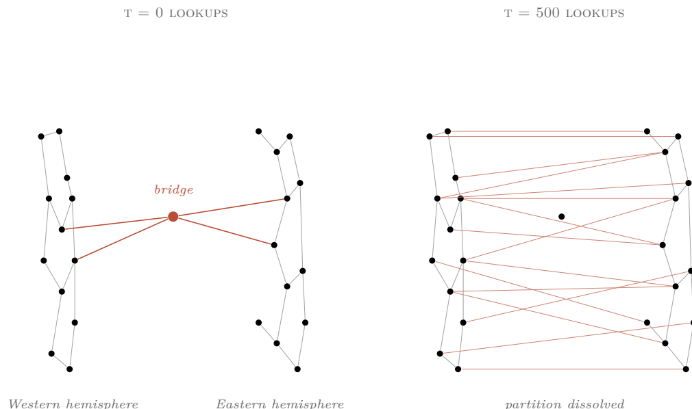
Figure 7: At t = 0 (left), the partition has a single bridge node connecting two hemispheres. By t = 500 lookups (right), hop caching has installed cross-hemisphere shortcuts in many intermediate nodes; triadic closure has converted observed transit pairs into direct edges. The bridge is no longer special. The protocol does not keep finding the bridge—it uses the bridge to rebuild the bridges that were cut.
